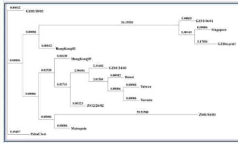
Fig. 1. Phylogenetic tree with maximum likelihood method
