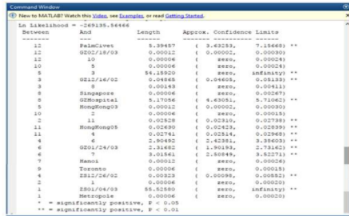
Fig. 2. Output of branch length and approximation confidence limits
