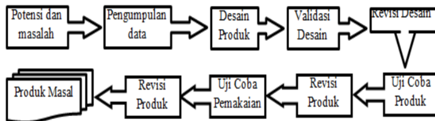
Gambar 1. Langkah-Langkah R&D
