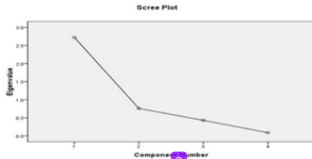
Gambar 1. Scree Plot
