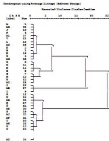
Gambar 4. Dendrogram Average Linkage APS
