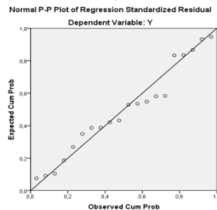
Gambar 1. Uji Kenormalan Residual
