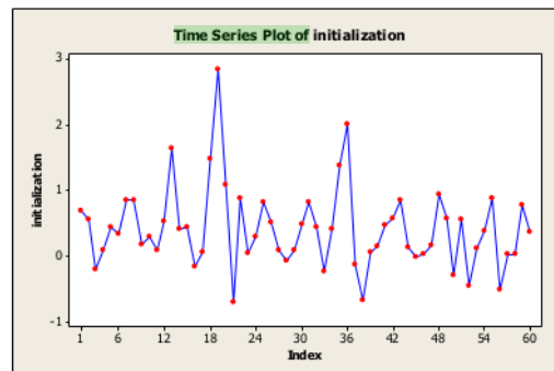
Gambar 1. Plot Time Series Data In Sample
